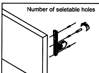
121 Front assembly
