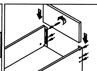
Back assembly
