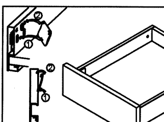
89 Front assembly
