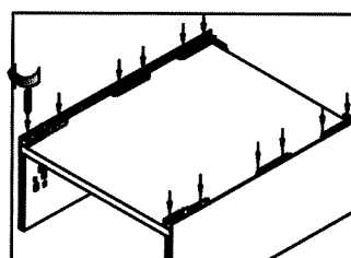
Bottom assembly
