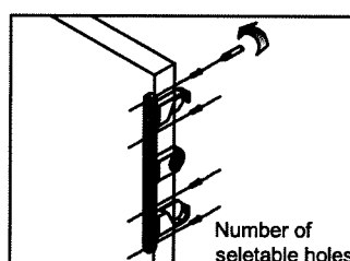
Front assembly
